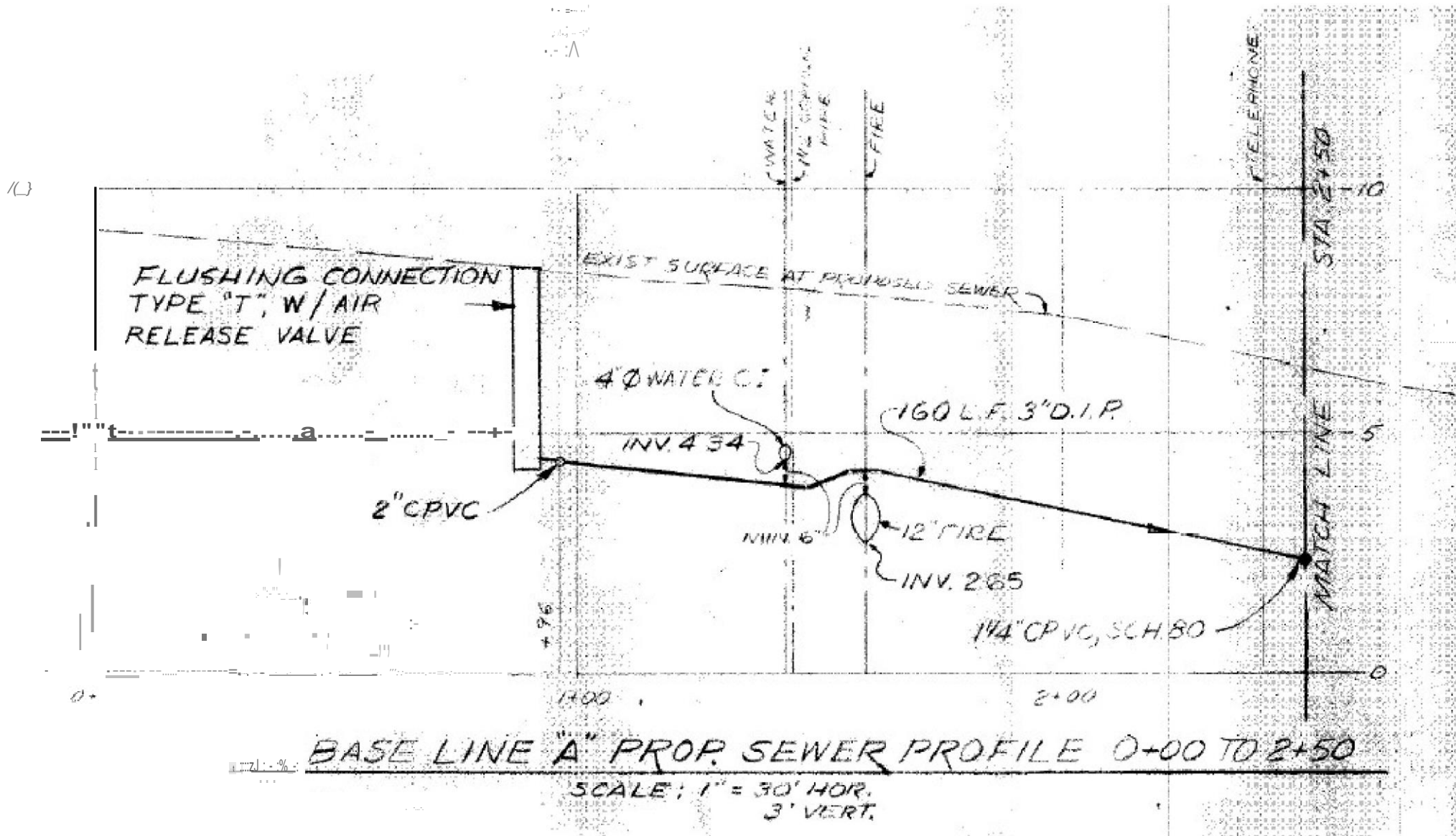
Building B Force Main Profile
