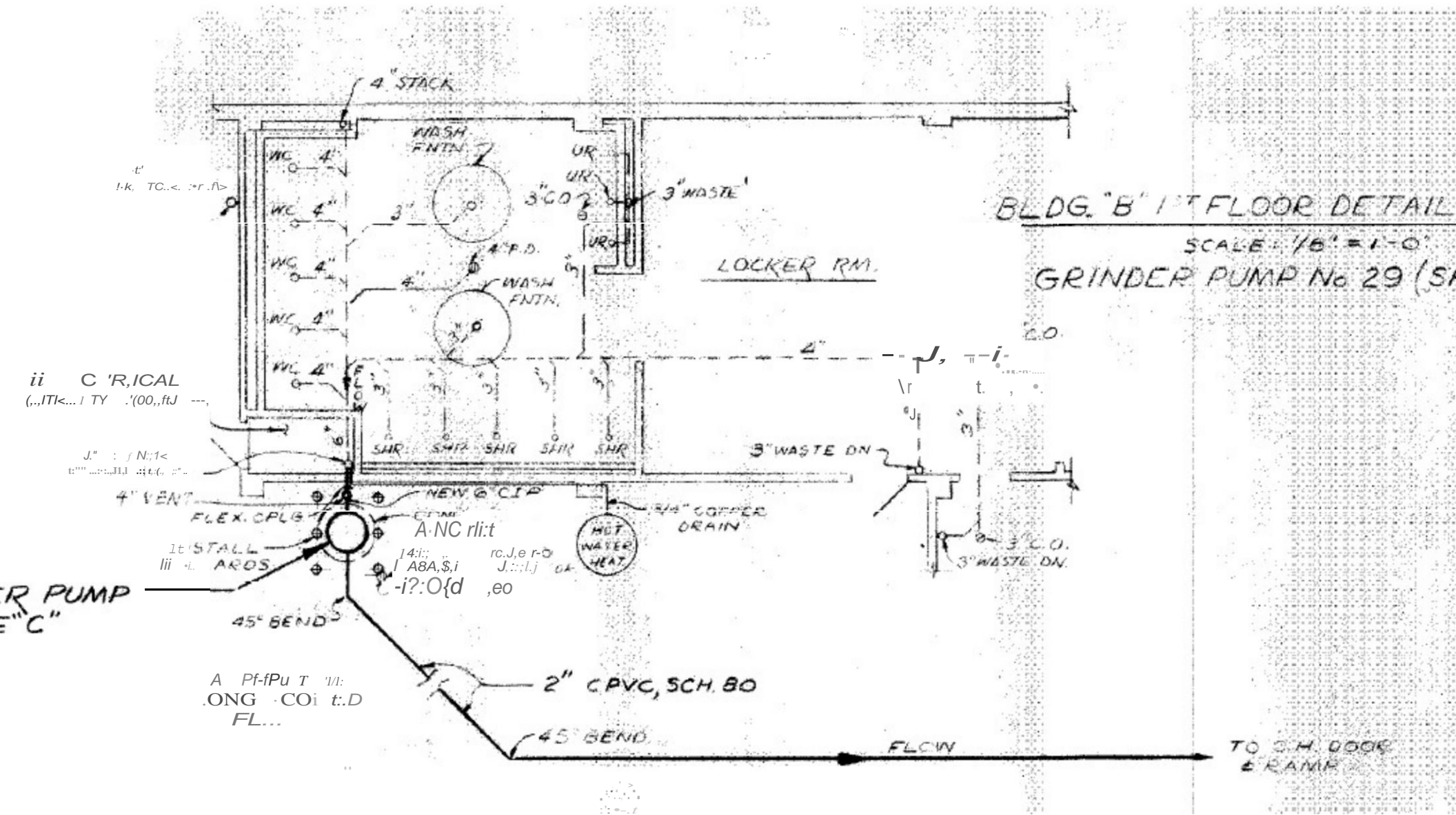
Building B Floor Plan
