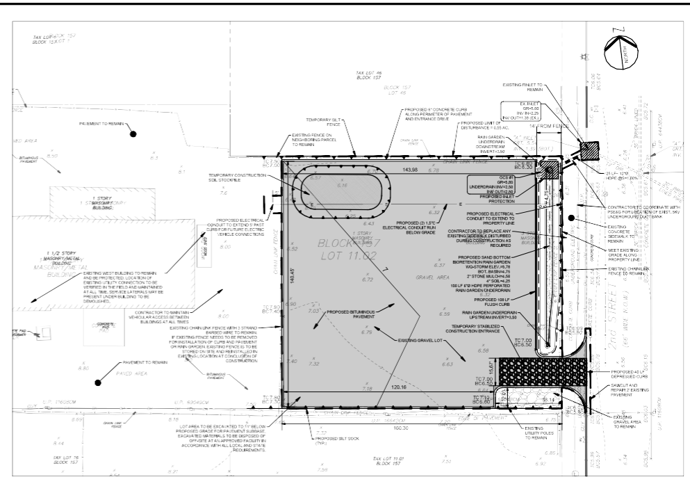
PROPOSED SITE, GRADING, DRAINAGE, UTILITY AND SOIL EROSION PLAN
