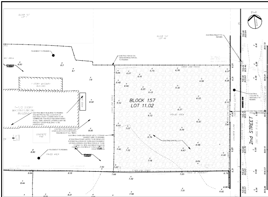
EXISTING CONDITIONS & DEMOLITION PLAN
