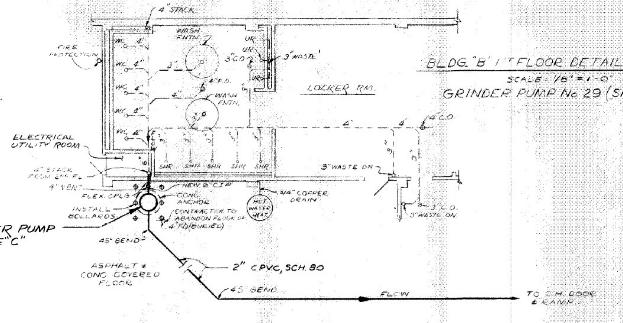
Building B Floor Plan
