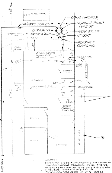
BLDG 'D' DETAIL PLAN (BECKETT) SCALE: 1"=10' GRINDER PUMP No. 26 (SHE)
