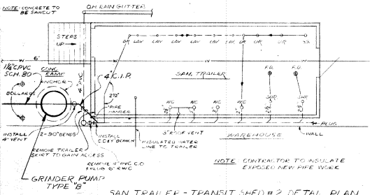
SAN TRAILER - TRANSIT SHED #2 DETAIL PLAN SCALE: 1/4" = 1'-0" GRINDER PUMP NO. 32
