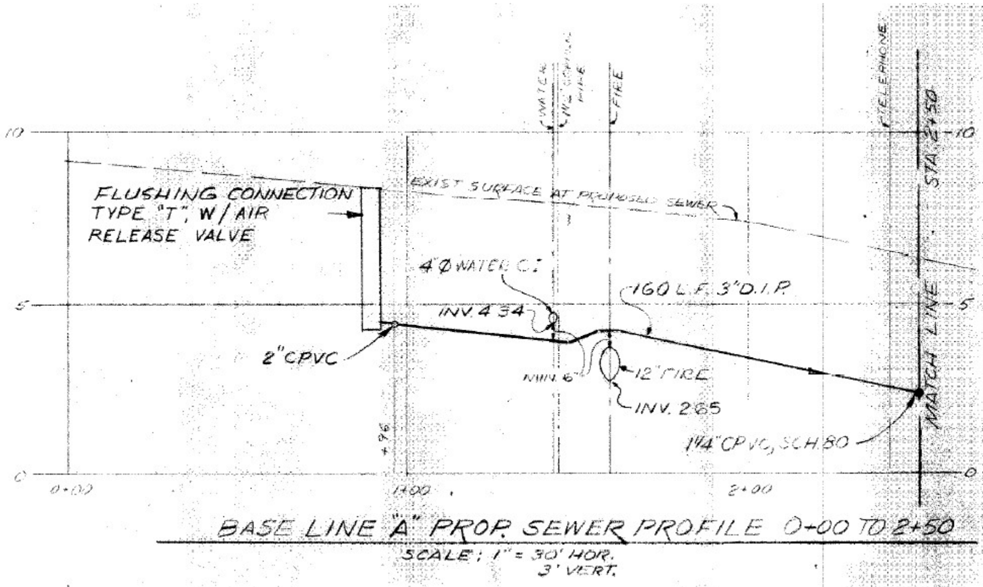
Building B Force Main Profile
